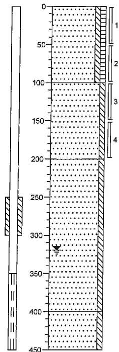
Boring: 05
