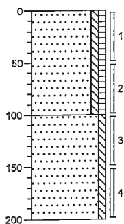
Boring: 01
